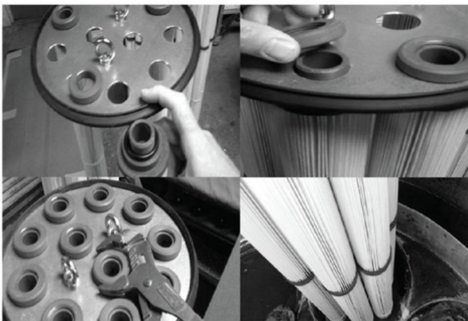
Assembly of a Jellyfish Filter cartridge (left) and installation of a filter cartridge into a cartridge receptacle in the deck (right).
